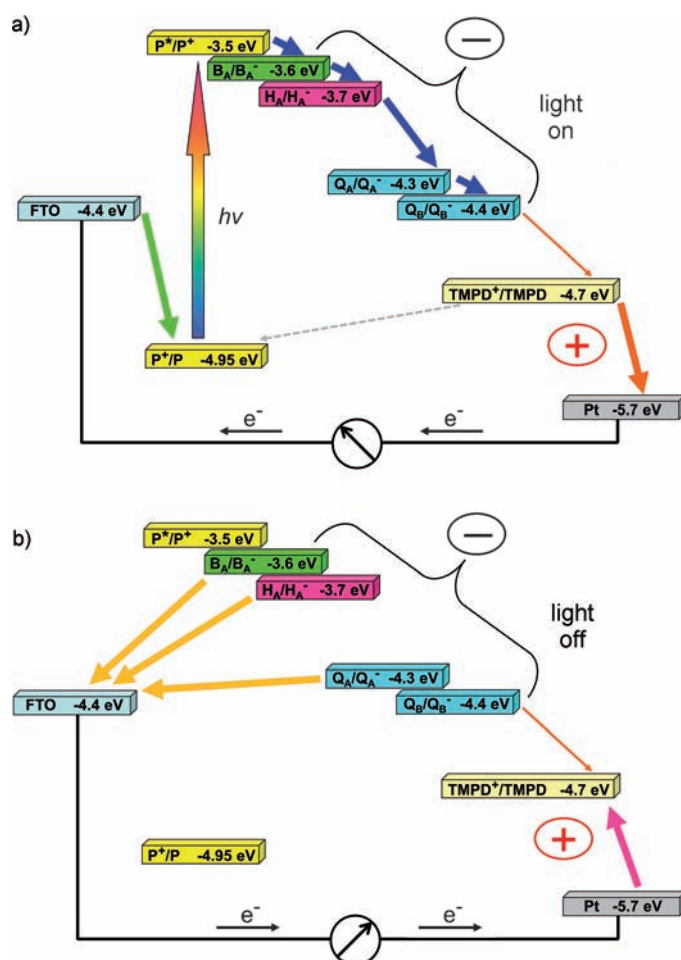
Figure 4. a) Proposed mechanism of current generation in the light. Photo-excitation in the RC (rainbow arrow) initiates charge separation in the RC (blue arrows); electrons are shuttled to the Pt electrode by TMPD (orange arrows); \text{P}^+ is reduced by the FTO-glass electrode (green arrow); limiting electron transfer from the RC to \text{TMPD}^+ (narrow orange arrow) causes an initial over-reduction of the RC cofactors and over-oxidation of the TMPD pool. b) Proposed mechanism of reverse electron flow after turning off the excitation light. Electrons are donated by the over-reduced RC cofactors to the FTO electrode (gold arrows), and the \text{TMPD}^+ pool is reduced by the Pt electrode (magenta arrow), thereby producing a transient reverse electron transfer until the potential difference is dissipated.
